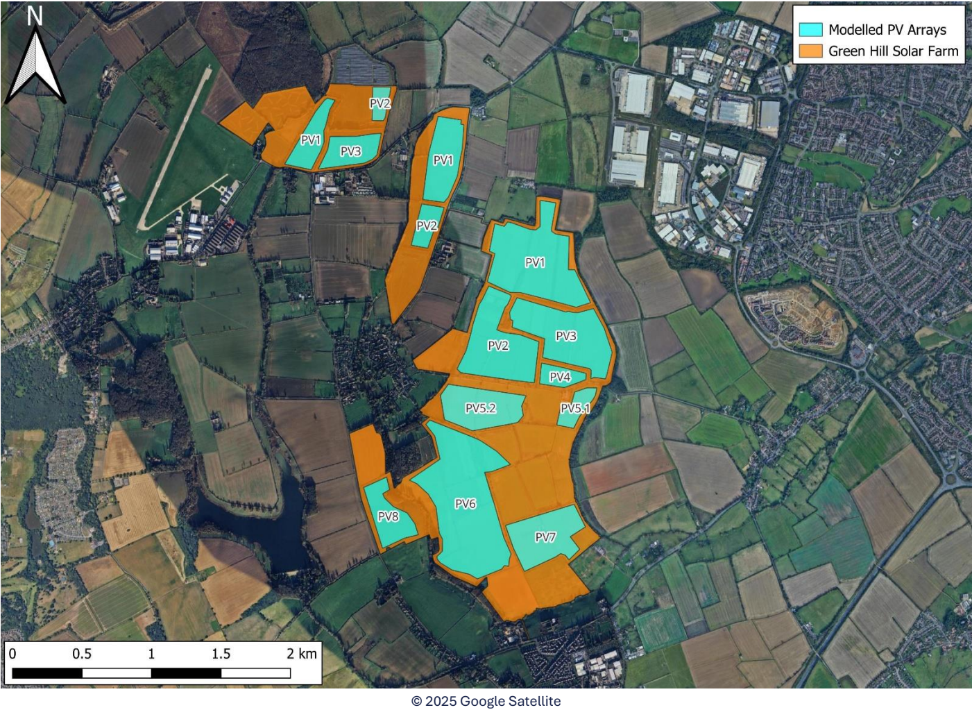
Figure 2.3: Modelled PV Panels at Green Hill C, Green Hill D, and Green Hill E
