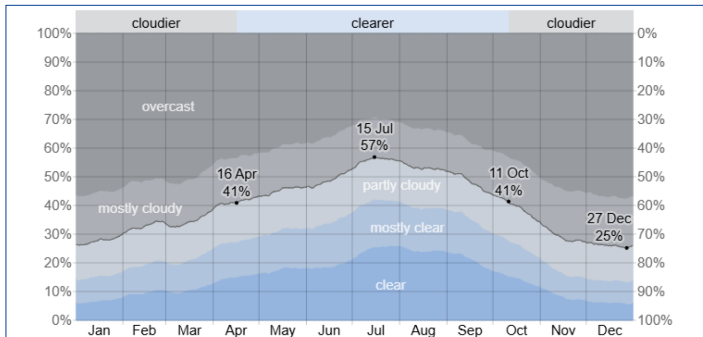
Figure 7.1: Cloud Cover at Earls Barton
